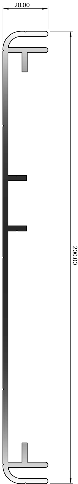
SECTION No. 35243 1.850 kg/m P = 599.95
