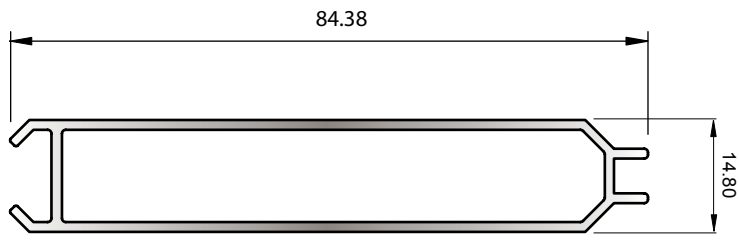
SECTION No. G824 0.671 kg/m P = 214.83
