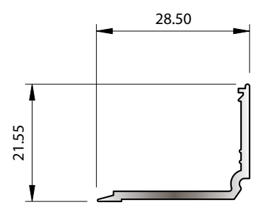
SECTION No. 34736 0.194 kg/m P = 100.54
