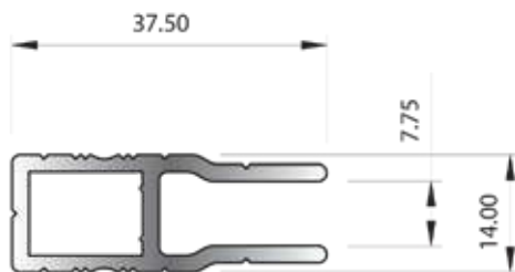
SECTION No. G253 ACCEPTS STAKING ANGLE X124L 0.500 kg/m P = 194.49
