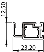
SECTION No. 30957 ACCEPTS STAKING ANGLE X429E 0.302 kg/m P = 117.77
