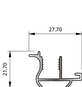
SECTION No. Z447 0.282 kg/m P = 165.46
