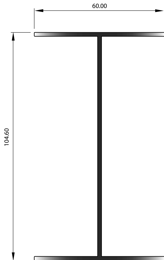
SECTION No. G902 1.078 kg/m P = 445.57
