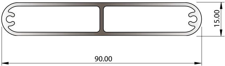
SECTION No. 31292 0.968 kg/m P = 197.12
