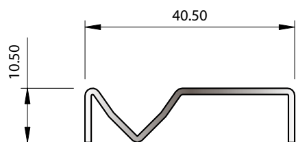
SECTION No. 9251 0.217 kg/m P = 136.10
