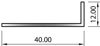
SECTION No. 7084 0.205 kg/m P = 104
