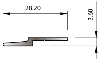
SECTION No. K805 0.116 kg/m P = 62.50
