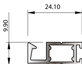
SECTION No. J058 ACCEPTS STAKING ANGLE X429E 0.232 kg/m P = 94.71
