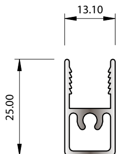
SECTION No. Z439 0.285 kg/m P = 106.40
