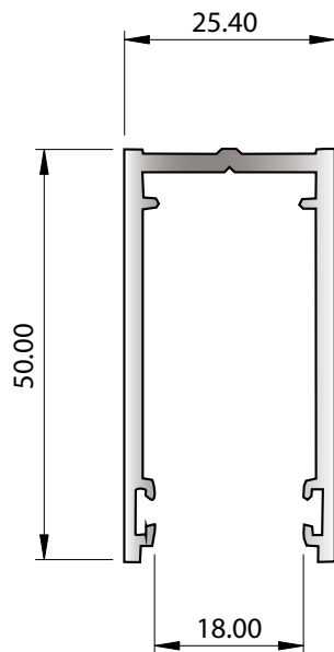
SECTION No. 33604 0.742 kg/m P = 275.99
