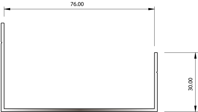
SECTION No. 31347 0.614 kg/m P = 304.48
