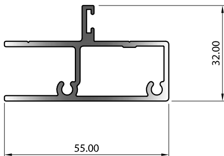
SECTION No. 37523 0.804 kg/m P = 237.92
