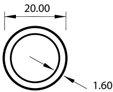
SECTION No. TU8240 0.251 kg/m P = 62.8
