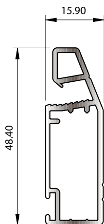
SECTION No. 31966 ACCEPTS STAKING ANGLE J688E 0.515 kg/m P = 156.98
