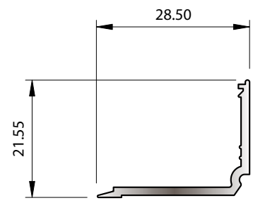
SECTION No. 34736 0.194 kg/m P = 100.54
