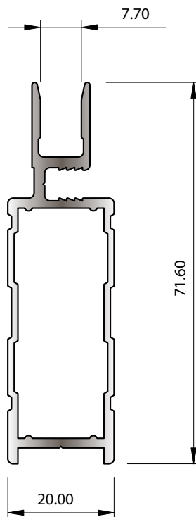
SECTION No. Z340 ACCEPTS STAKING ANGLE 6868E 0.751 kg/m P = 240.51
