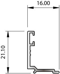
SECTION No. 34733 0.132 kg/m P = 88.11
