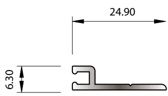
SECTION No. X389 0.139 kg/m P = 71.64
