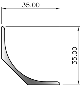
SECTION No. 7789 0.360 kg/m P = 118.32
