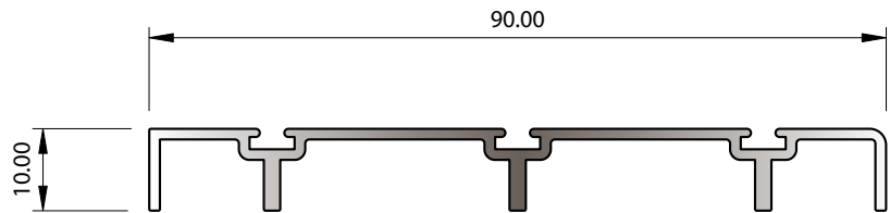
SECTION No. 33957 0.543 kg/m P = 290.37
