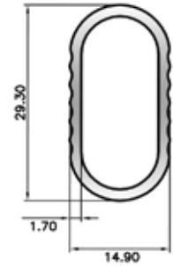
SECTION No. 36157 0.310 kg/m P = 76.58
