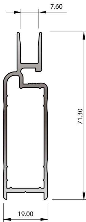
SECTION No. 33423 ACCEPTS STAKING ANGLE 6868K 0.744 kg/m P = 227.67
