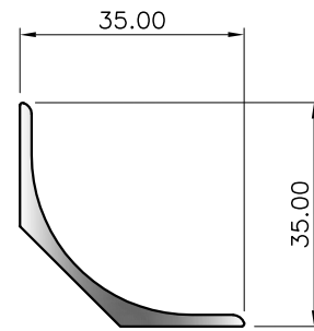
SECTION No. 7789 0.360 kg/m P = 118.32
