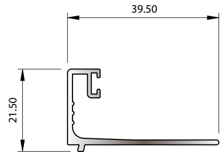
SECTION No. 36117 0.275 kg/m P = 155.35
