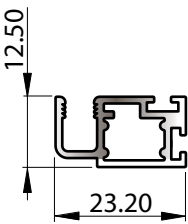
SECTION No. 30957 ACCEPTS STAKING ANGLE X429E 0.302 kg/m P = 117.77
