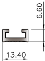
SECTION No. 36404 0.121 kg/m P = 56.06
