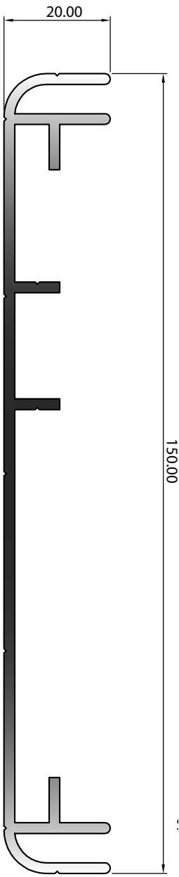
SECTION No. 35242 1.346 kg/m P = 503.49
