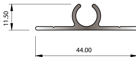
SECTION No. 8955 0.279 kg/m P = 129.99
