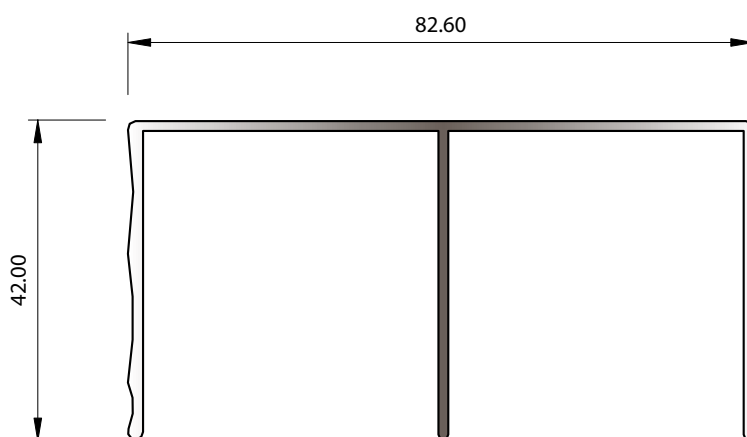
SECTION No. N924 0.745 kg/m P = 409.90
