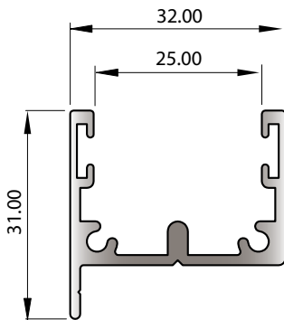
SECTION No. 33627 0.483 kg/m P = 217.96 LENGTH = 4.6m
