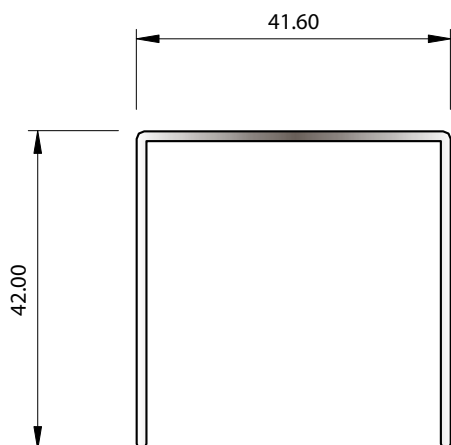
SECTION No. 9250 0.431 kg/m P = 246.63
