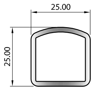
SECTION No. 34069 0.459 kg/m P = 91.18
