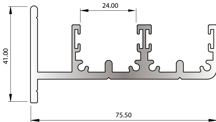
SECTION No. 34689 1.521 kg/m P = 453.62 LENGTH = 4.6m
