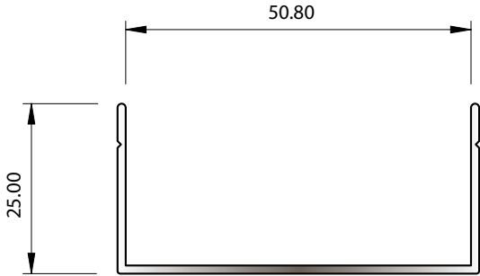
SECTION No. 9056 0.324 kg/m P = 203.00
