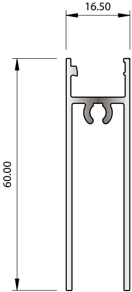
SECTION No. 33959 0.592 kg/m P = 292.46
