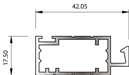
SECTION No. 9775 ACCEPTS STAKING ANGLE J688E 0.494 kg/m P = 150.10
