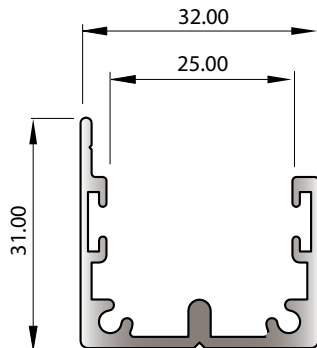
SECTION No. 33629 0.483 kg/m P = 217.75 LENGTH = 4.6m
