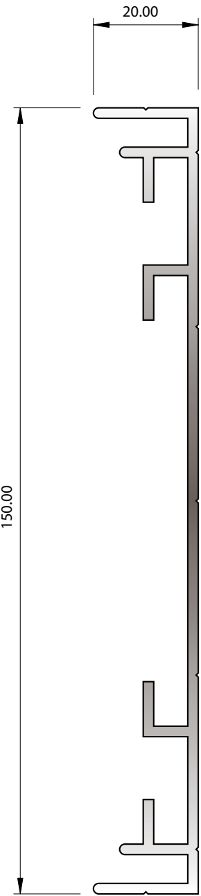
SECTION No. X540 1.418 kg/m P = 528.89
