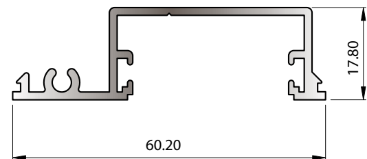
SECTION No. 30771 0.511 kg/m P = 247.49
