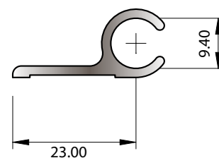
SECTION No. 6595 0.221 kg/m P = 95.94
