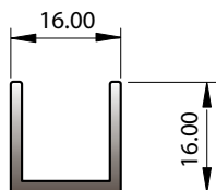
SECTION No. 5979 0.194 kg/m P = 92.80
