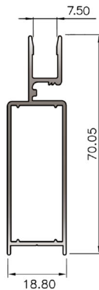
SECTION No. 31701 0.589 kg/m P = 230.62 ACCEPTS STAKING ANGLE 6868L
