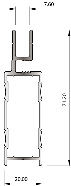
SECTION No. Z785 ACCEPTS STAKING ANGLE 6868K 0.748 kg/m P = 240.25
