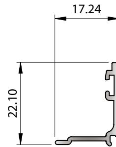
SECTION No. 33605 0.160 kg/m P = 91.28
