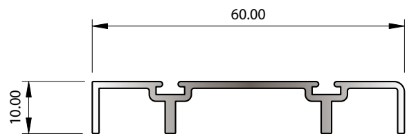
SECTION No. 33956 0.382 kg/m P = 205.55
