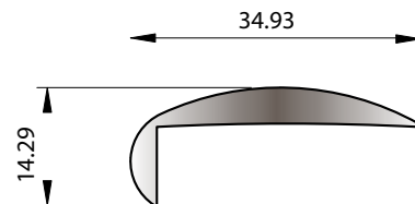
SECTION No. 0330 0.342 kg/m P = 88
