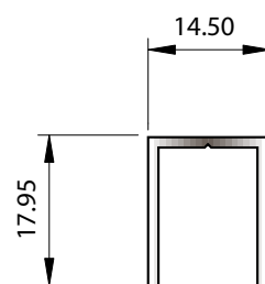
SECTION No. X075 0.162 kg/m P = 98.63
