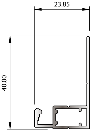
SECTION No. 34918 ACCEPTS STAKING ANGLE X429E 0.325 kg/m P = 143.76
