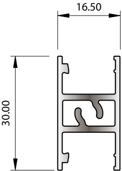
SECTION No. 33958 0.391 kg/m P = 140.03
