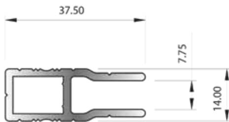
SECTION No. G253 ACCEPTS STAKING ANGLE 662117 0.500 kg/m P = 194.49
