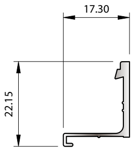
SECTION No. 34734 0.148 kg/m P = 86.26
