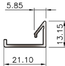
SECTION No. 36405 0.154 kg/m P = 87.09
