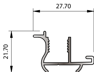
SECTION No. Z447 0.282 kg/m P = 165.46
