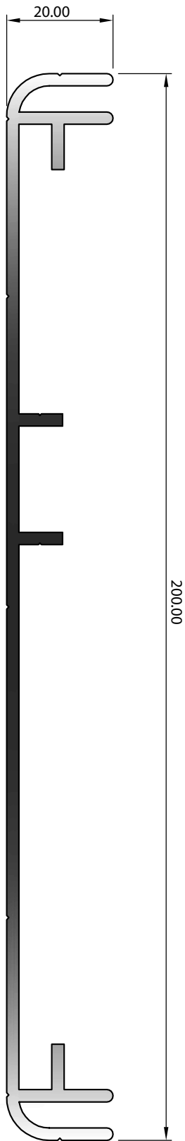
SECTION No. 35243 1.850 kg/m P = 599.95
