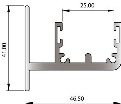
SECTION No. 33628 0.936 kg/m P = 295.94 LENGTH = 4.6m
