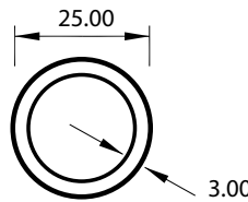
SECTION No. TU8575 0.562 kg/m P = 78.5
