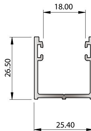
SECTION No. 33602 0.353 kg/m P = 178.41
