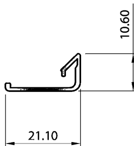
SECTION No. 37488 0.109 kg/m P = 77.13
