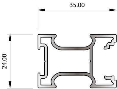
SECTION No. 33960 0.516 kg/m P = 199.03
