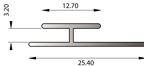
SECTION No. 34378 0.089 kg/m P = 82.83 2x scale
