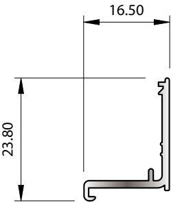
SECTION No. 34732 0.154 kg/m P = 90.09
