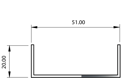
SECTION No. 6330 0.370 kg/m P = 185
