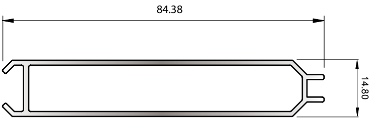
SECTION No. G824 0.671 kg/m P = 214.83
