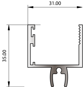
SECTION No. 34244 0.501 kg/m P = 222.81
