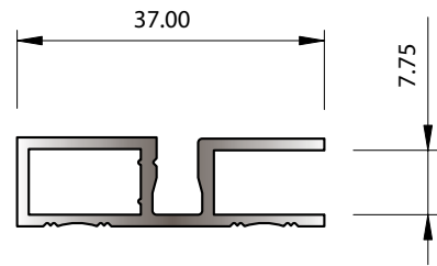
SECTION No. 5663 ACCEPTS STAKING ANGLE X124G 0.351 kg/m P = 143.50
