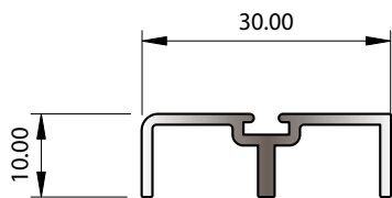
SECTION No. 33955 0.220 kg/m P = 120.72
