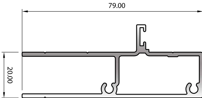
SECTION No. J007D 1.022 kg/m P = 320.58
