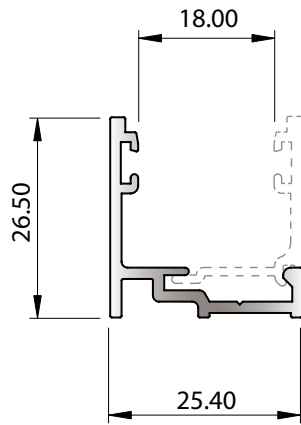
SECTION No. 33603 0.278 kg/m P = 141.75
