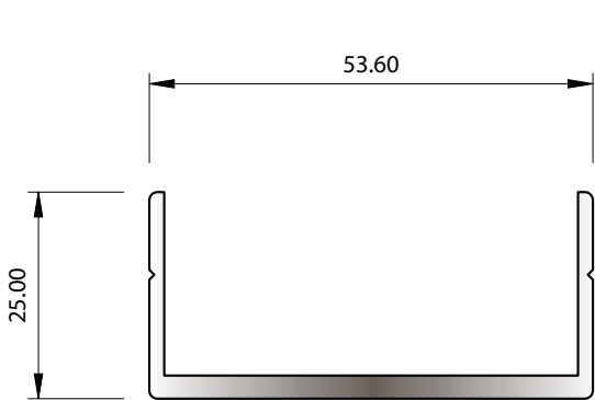
SECTION No. 7414 0.620 kg/m P = 200.87
